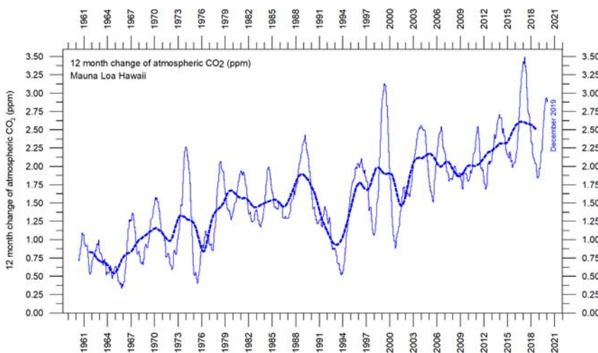
Figure 14: Growth in CO 2 concentration. Annual (12-month) growth rate (ppm) of atmospheric CO 2 since 1959, calculated as the average amount of atmospheric CO 2 during the last 12 months, minus the average for the preceding 12 months. The graph is based on data measured at the Mauna Loa Observatory, Hawaii. The thin blue line shows the value calculated month by month, while the dotted blue line represents the simple running 3-year average.
