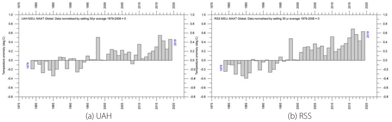
Figure 4: Global mean annual lower troposphere air temperatures since 1979.
