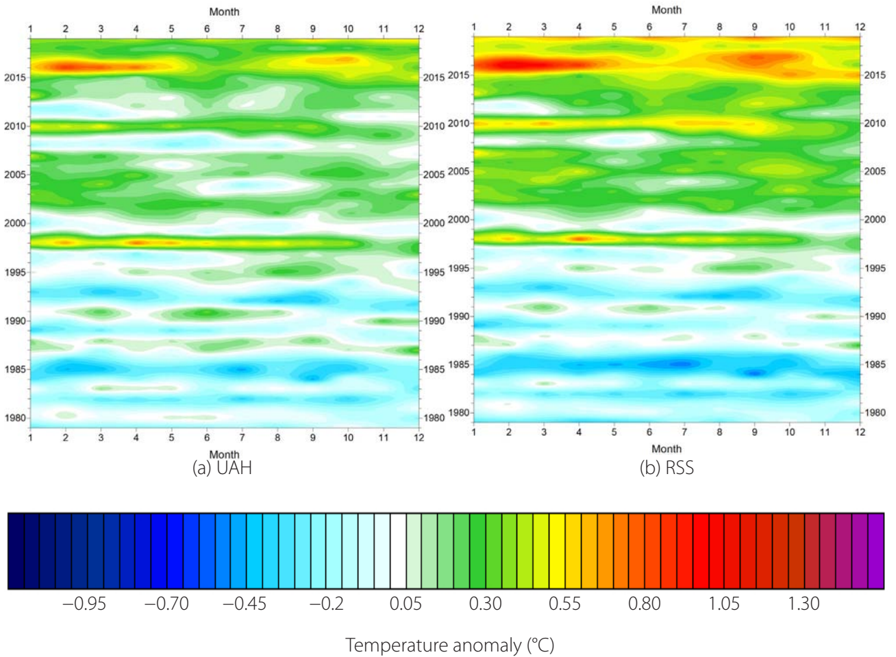
Figure 5: Temporal evolution of global lower troposphere temperatures since 1979.
