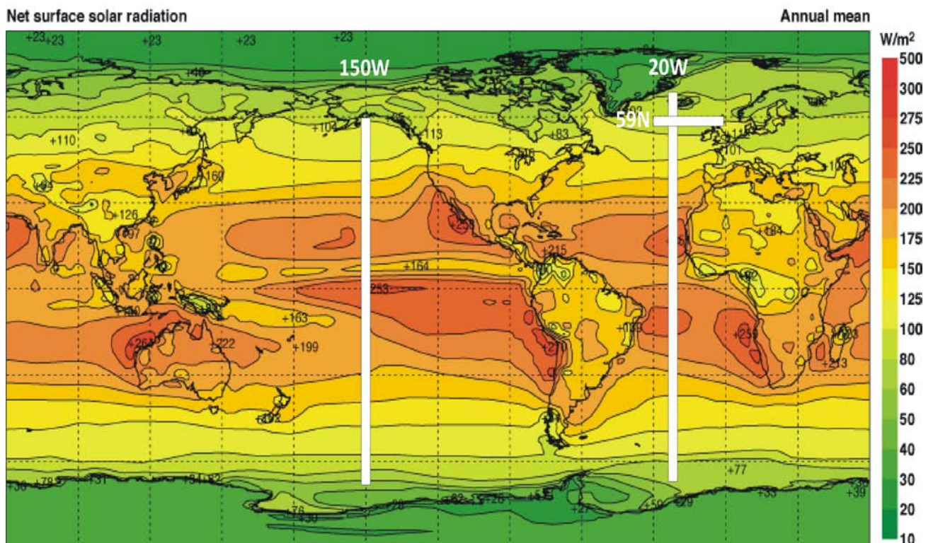
Figure 25: Annual mean net surface solar radiation ( \text{W}/\text{m}^2 ), and the location of three profiles.
