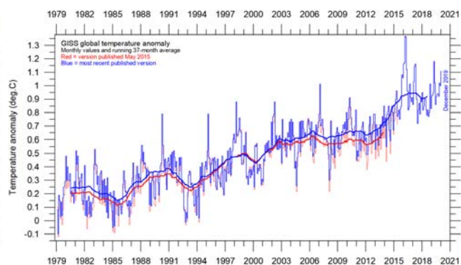
(c) GISS
