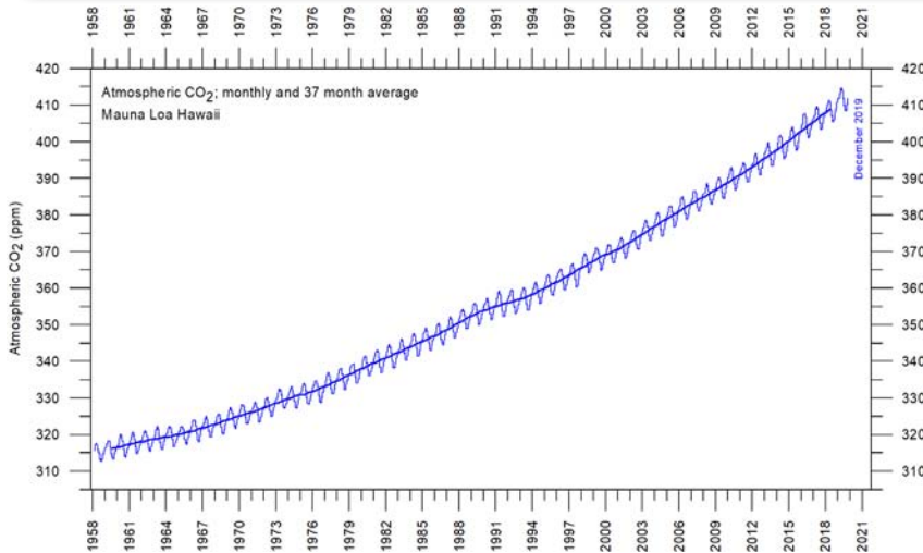
Figure 13: CO 2 concentration. Monthly amount of atmospheric CO 2 since March 1958, measured at the Mauna Loa Observatory, Hawaii. The thin line shows the monthly values, while the thick line is the simple running 37-month average, nearly corresponding to a running 3-year average.
