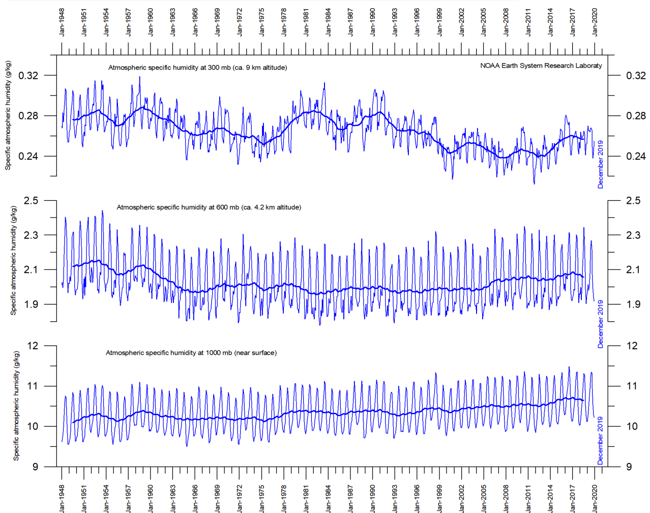
Figure 12: Humidity.
