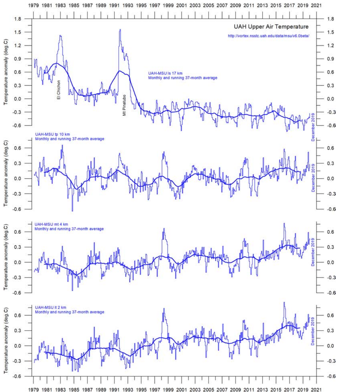
Figure 11: Temperatures by altitude.
