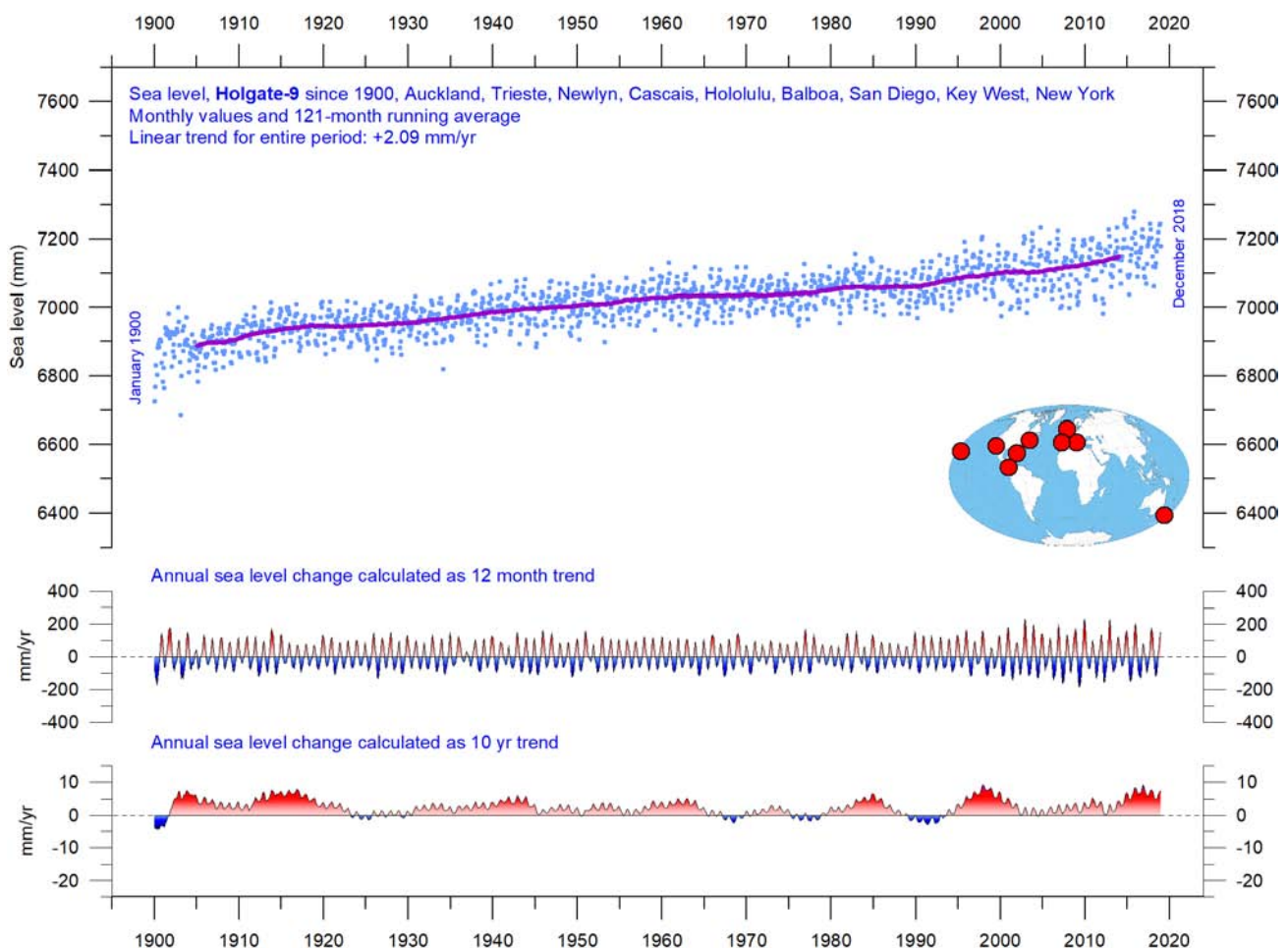
Figure 33: Holgate-9 monthly tide gauge data.
