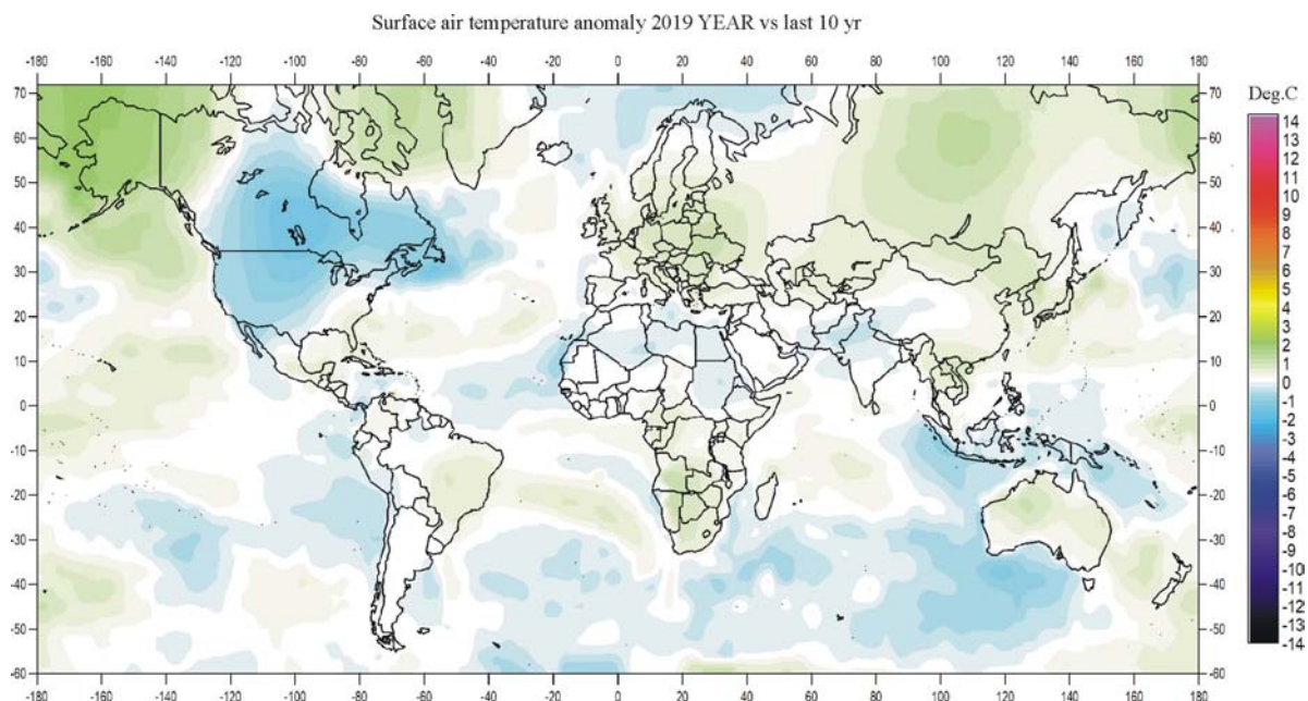
Figure 1: 2019 surface air temperatures compared to the average for the previous 10 years.
