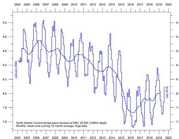
Figure 27: Temperature profile across the North Atlantic current.
