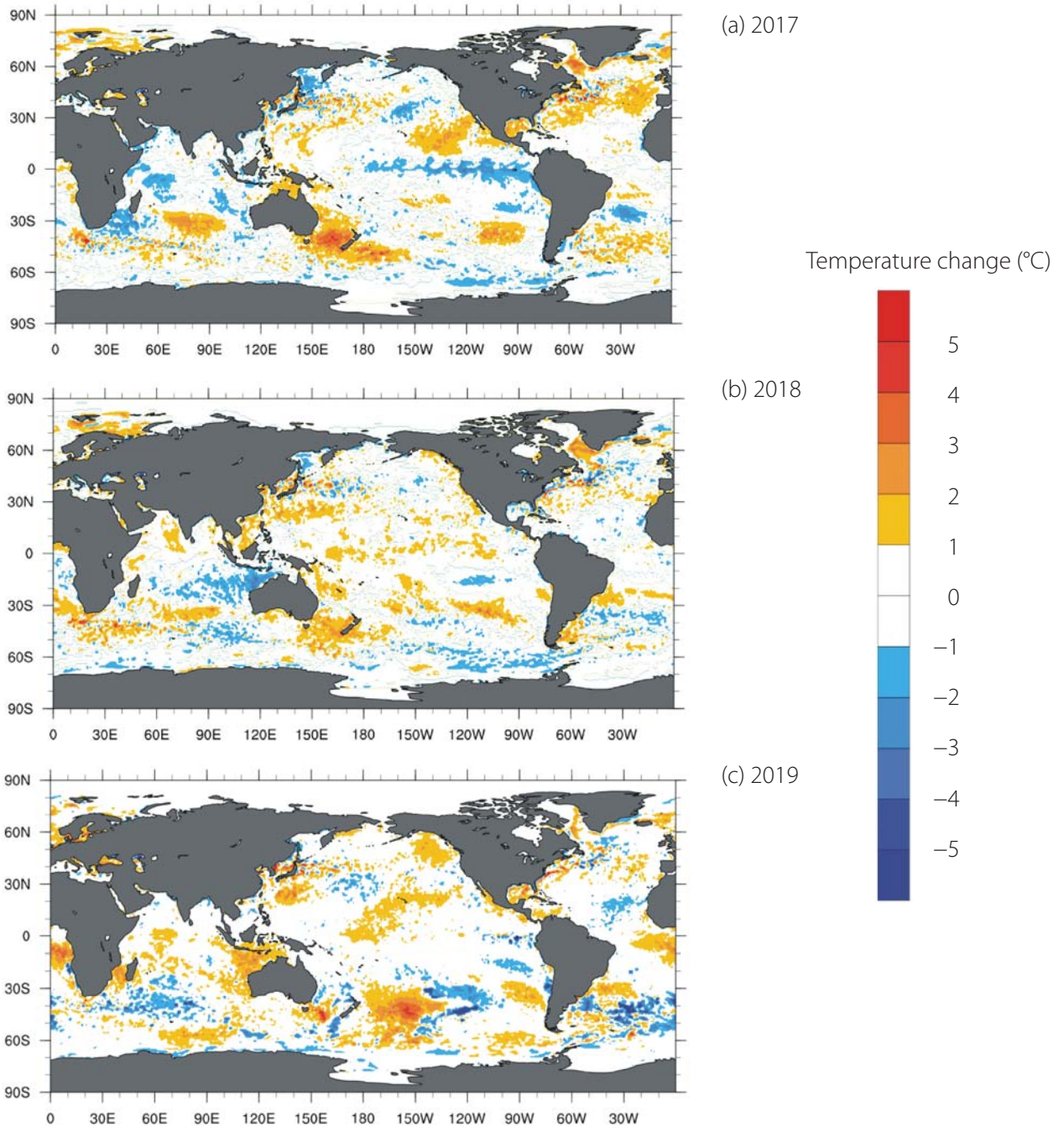
Figure 19: Spatial patterns of ocean surface temperatures, 2017–2019.
