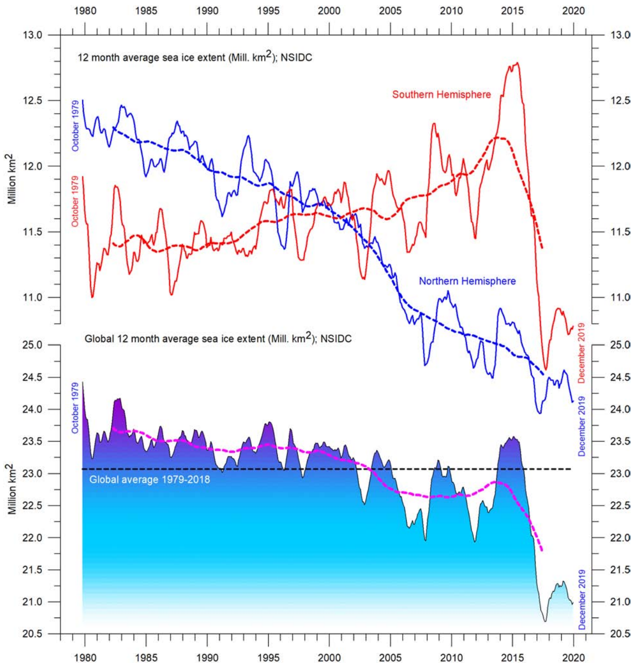
Figure 35: Global and hemispheric 12-month running average sea-ice extent since 1979.
