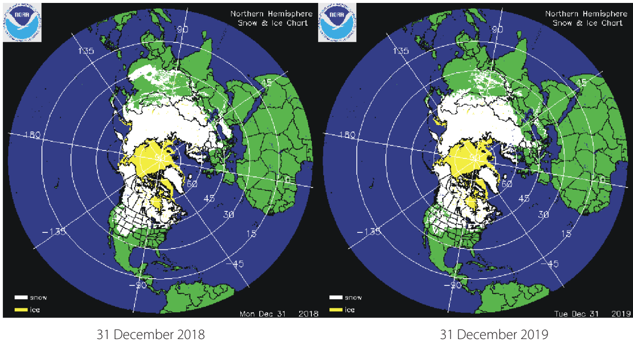
Figure 37: Arctic sea-ice extent and thickness.
