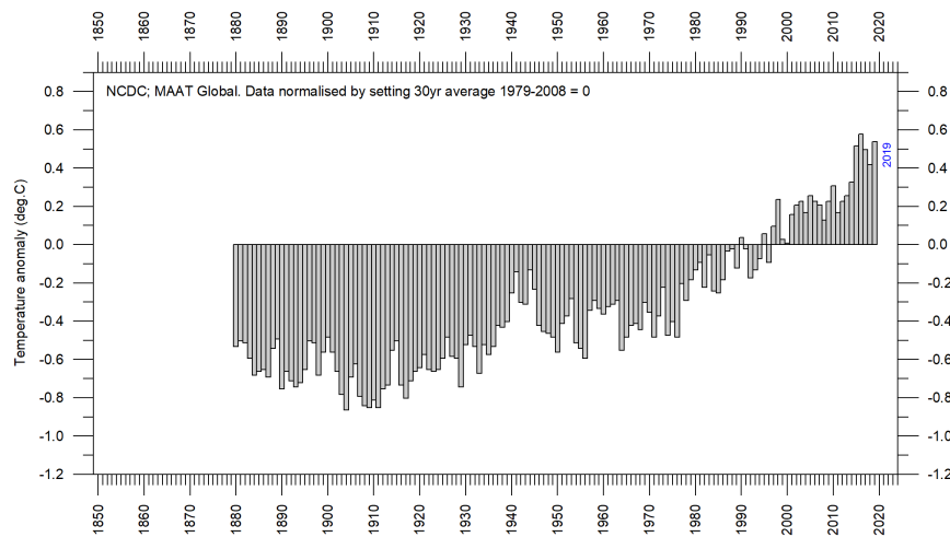
(b) NCDC
