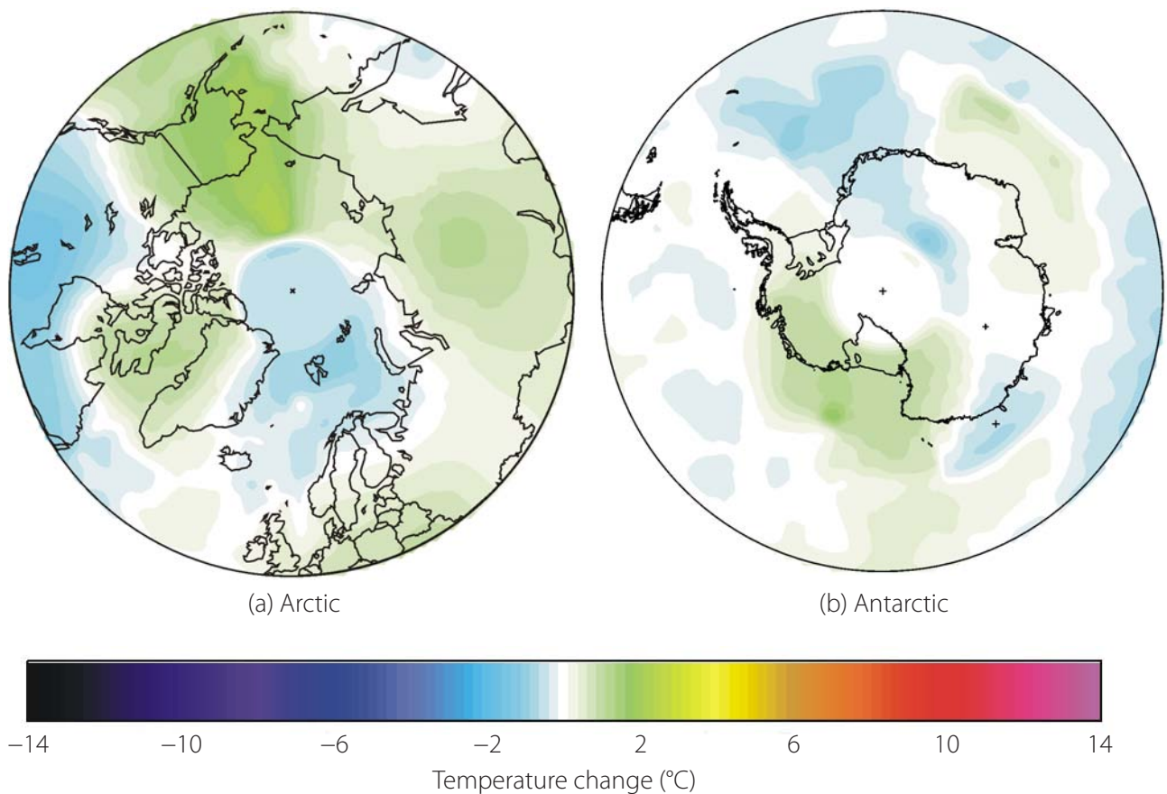
Figure 2: 2019 polar surface air temperatures compared to the average for the previous 10 years.
